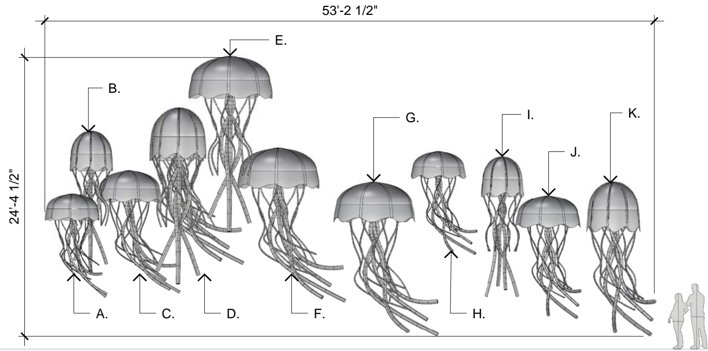
1 JELLIES ELEVATION FRONT SCALE: 1:100
